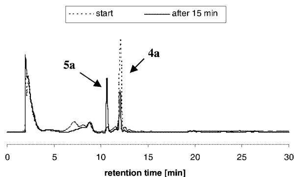
Figure 3. Cell extract incubation of AM- cycloSal -d4TMP triester 4a followed by HPLC (HPLC method: HPLC analysis method II was performed as reported in ref. [7] ).
