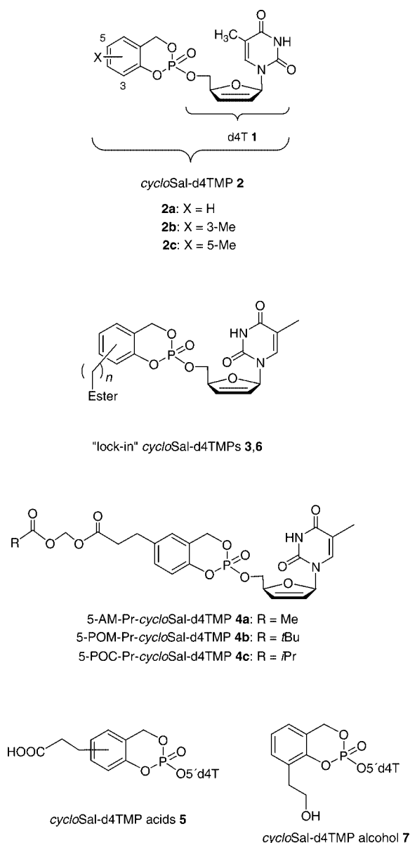
Scheme 1. Target cycloSal pronucleotides 3–7 of d4T 1.
