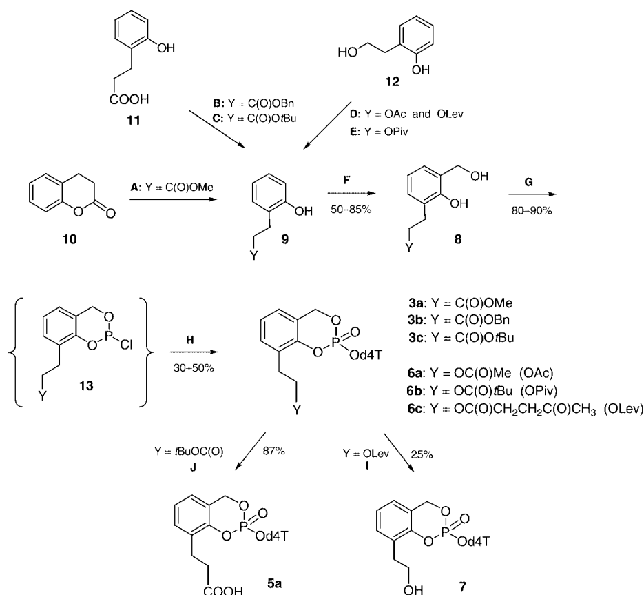
Scheme 2. Synthesis of the corresponding salicyl alcohols and the target triesters 3 , 5 , 6 and 7 . Method A : methanol, H 2 SO 4 , reflux, 5–8 h; method B : benzyl bromide, DBU, toluene, reflux, 7 h; method C : (CH 3 ) 2 NCH(OCH 2 tBu) 2 , tert -butyl alcohol, toluene, reflux, 5 h; method D : ethyl acetate or ethyl levulinate, n -hexane, SiO 2 ·NaHSO 4 , 67 °C, 6–18 h; method E : 3-pivaloyl-1,3-thiazolidine-2-thione, toluene, 65 °C, 48 h; method F : i) phenylboronic acid, propionic acid (cat.), p -formaldehyde, toluene, reflux, 6–8 h; ii) H 2 O 2 , THF, 0 °C, 30 min; method G : PCl 3 , pyridine, Et 2 O, 0–21 °C, 1 h; method H : i) d4T 1 , CH 3 CN, DIPEA, 0–20 °C; ii) t BuOOH, CH 3 CN, room temp., 30 min; method I : NH 2 NH 2 ·H 2 O, pyridine/HOAc (3:2), pyridine, 0 °C, 10 min; method J : TFA (10 equiv.), CH 2 Cl 2 , room temp., 1 h.
