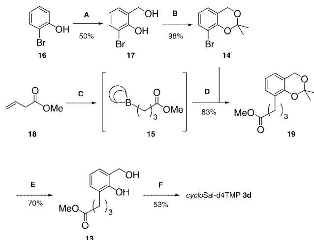
Scheme 3. Synthesis of the ester-functionalised cycloSal -d4TMP triester 3d with a C 3 linker. Method A: i) phenylboronic acid, propionic acid, (CH 2 O) n , toluene, reflux, 18 h; ii) H 2 O 2 , THF, 0 °C, 45 min; method B: 2,2-dimethoxypropane, p TsOH, acetone, Na 2 SO 4 ; method C: 9-BBN, THF, 0 °C → 55 °C, 16 h; method D: K 2 CO 3 , [Pd(dppf)Cl 2 ], DMF, 55 °C, 4 d; method E: cat. HCl, CH 3 CN/H 2 O, 5 min; method F: i) PCl 3 , pyridine, Et 2 O, –20 °C to room temp., 2 h; ii) 1 , DIPEA, CH 3 CN, –20 °C to room temp., 1 h; iii) t BuOOH, CH 3 CN, –20 °C to room temp., 1 h.
