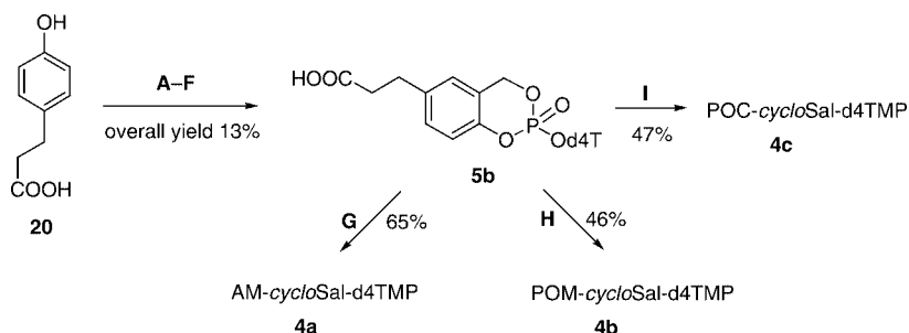
Scheme 4. Synthesis of enzyme-cleavable 5-functionalised cycloSal -d4TMP triesters 4 . Method A: (CH 3 ) 2 NCH(OCH 2 t Bu) 2 , tert -butyl alcohol, toluene, reflux, 5 h; method B: i) phenylboronic acid, propionic acid (cat.), p -formaldehyde, toluene, reflux, 6–8 h; ii) H 2 O 2 , THF, 0 °C, 30 min; method C: PCl 3 , pyridine, Et 2 O, 0–21 °C, 1 h; method D: i) d4T 1 , CH 3 CN, DIPEA, 0–20 °C; ii) t BuOOH, CH 3 CN, room temp., 30 min; method F: TFA (10 equiv.), CH 2 Cl 2 , room temp., 1 h; method G: bromomethyl acetate, DIPEA, CH 3 CN, 10 °C, 3 h; method H: chloromethyl acetate, DIPEA, CH 3 CN, room temp., 9 d; method I: chloromethyl isopropyl carbonate, DIPEA, CH 3 CN, 50 °C, 7 d.
