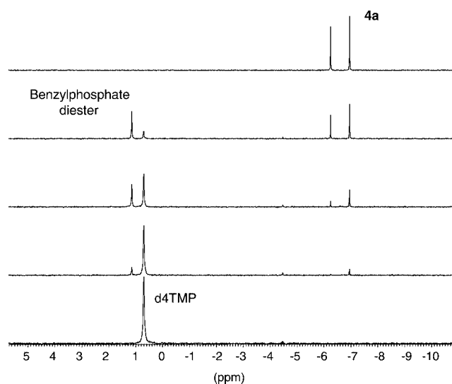
Figure 2. Chemical hydrolysis of the AM- cycloSal -d4TMP triester 4a followed by 31 P NMR spectroscopy {solvent: [D 6 ]DMSO/50 mM imidazole·HCl buffer (pH = 7.3), 1:1 (v/v); spectra were recorded once a week; H 3 PO 4 was used as external reference}.
